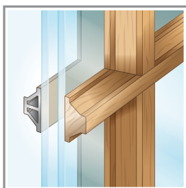
CLASSIC DIVIDED LIGHTS*
