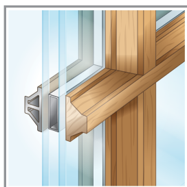
MODERN DIVIDED LIGHTS*
